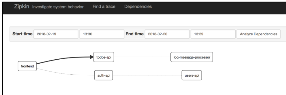
Figure 7: Sample Dependency Graph
